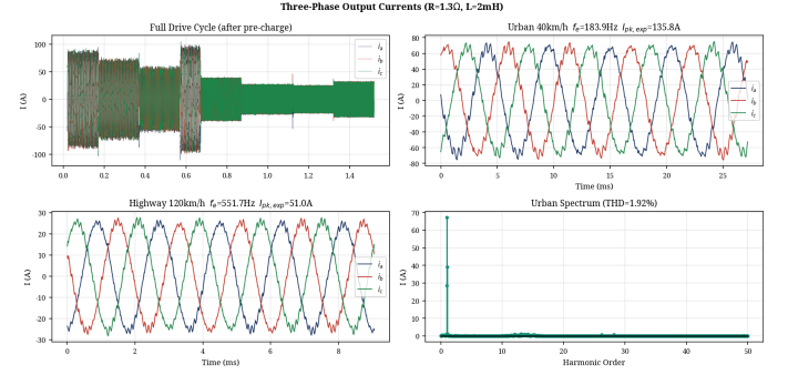
Fig. 2. Three-phase output currents and the harmonic spectrum during the urban driving segment.
