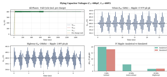
Fig. 1. Flying Capacitor voltage balancing demonstrating the 20ms pre-charge transient and steady-state ripple at urban and highway speeds.
