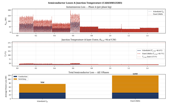
Fig. 3. Instantaneous semiconductor losses and junction temperature comparison between the scheduled and fixed switching frequencies.
