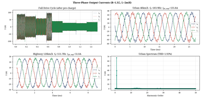
Fig. 4. Simulated three-phase output currents demonstrating proper sinusoidal synthesis.
