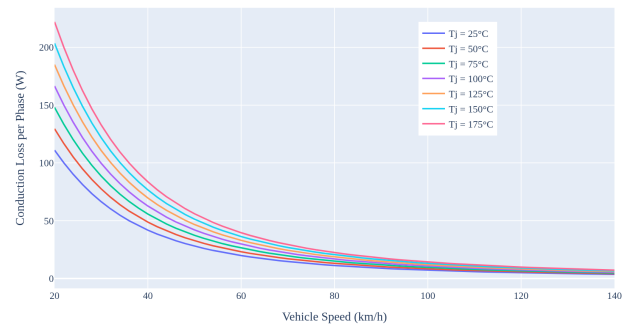
Conduction Loss vs Vehicle Speed at Various Junction Temperatures CAB450M12XM3: R_{ds\_on} = 3.3m\Omega (25°C) to 6.6m\Omega (175°C)
