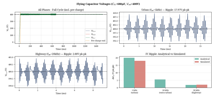
Fig. 6. Flying Capacitor voltage balancing demonstrating the 20ms pre-charge transient and steady-state ripple at urban and highway speeds.
