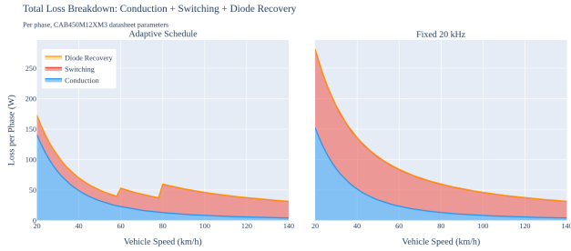
Fig. 3. Breakdown of conduction, switching, and diode recovery losses comparing the adaptive schedule against a fixed 20 kHz baseline.
