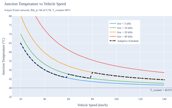
Fig. 7. Junction temperature vs vehicle speed, demonstrating the thermal safety margin of the adaptive schedule compared to fixed frequencies.
