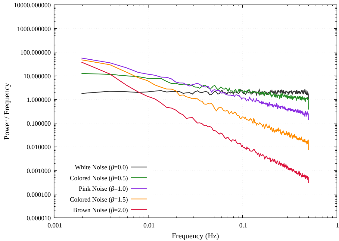
Power Spectral Density (PSD) of Colored Observation Noise
