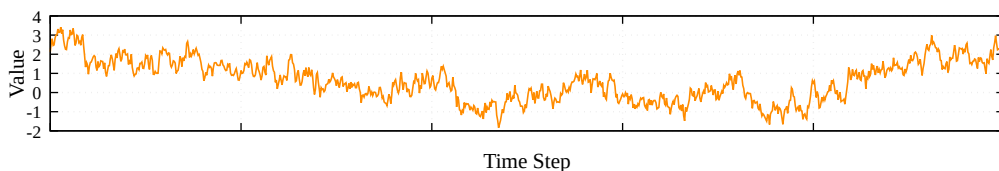
Brown/Red Noise ( \beta=2.0 )
