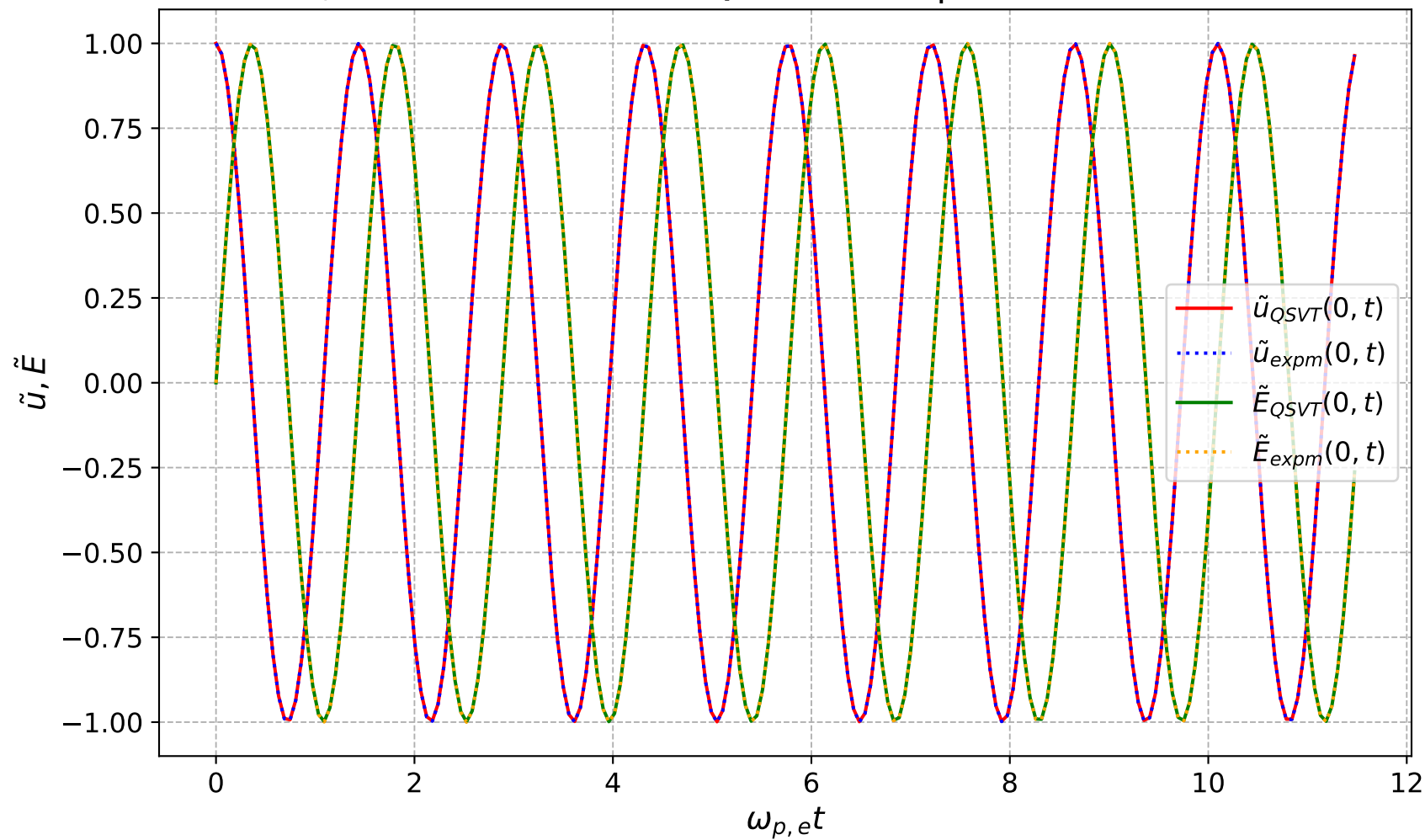
u,E of discretized KvN-QSVT and expm at x=0 vs time
