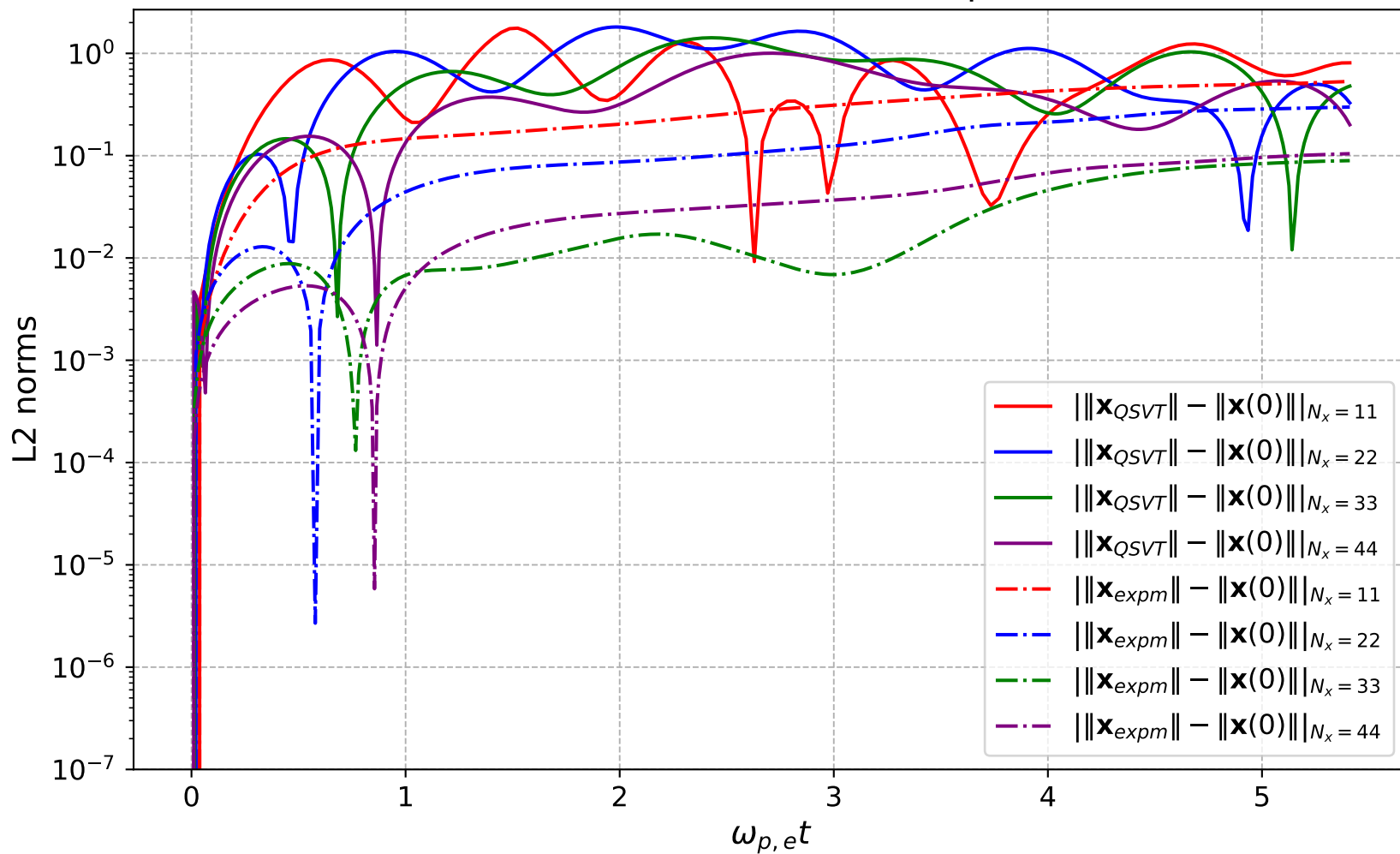
Deviation Errors of discretized KvN-QSVT and expm vs time with various N_x
