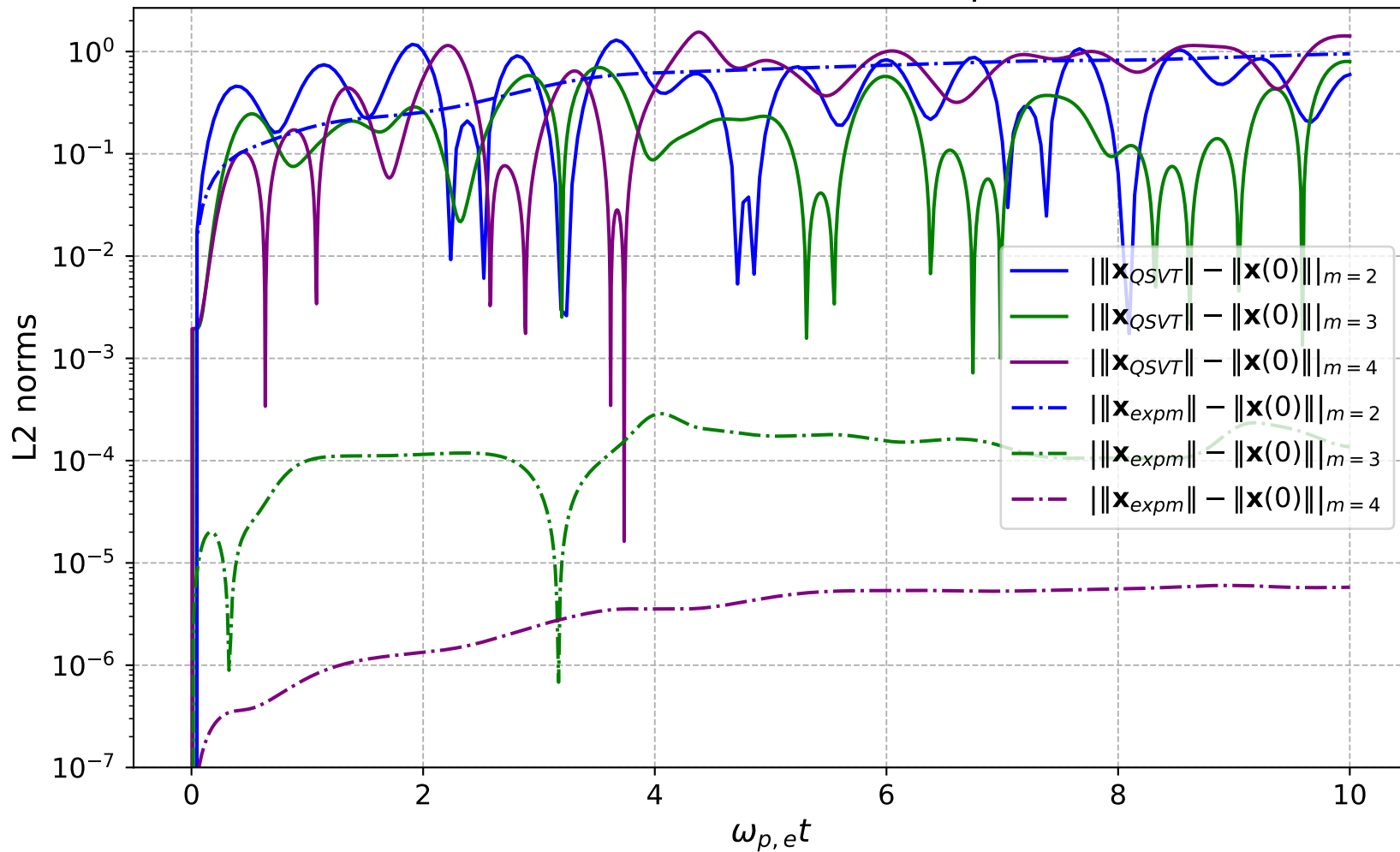
Deviation Errors of discretized KvN-QSVT and expm vs time with various m
