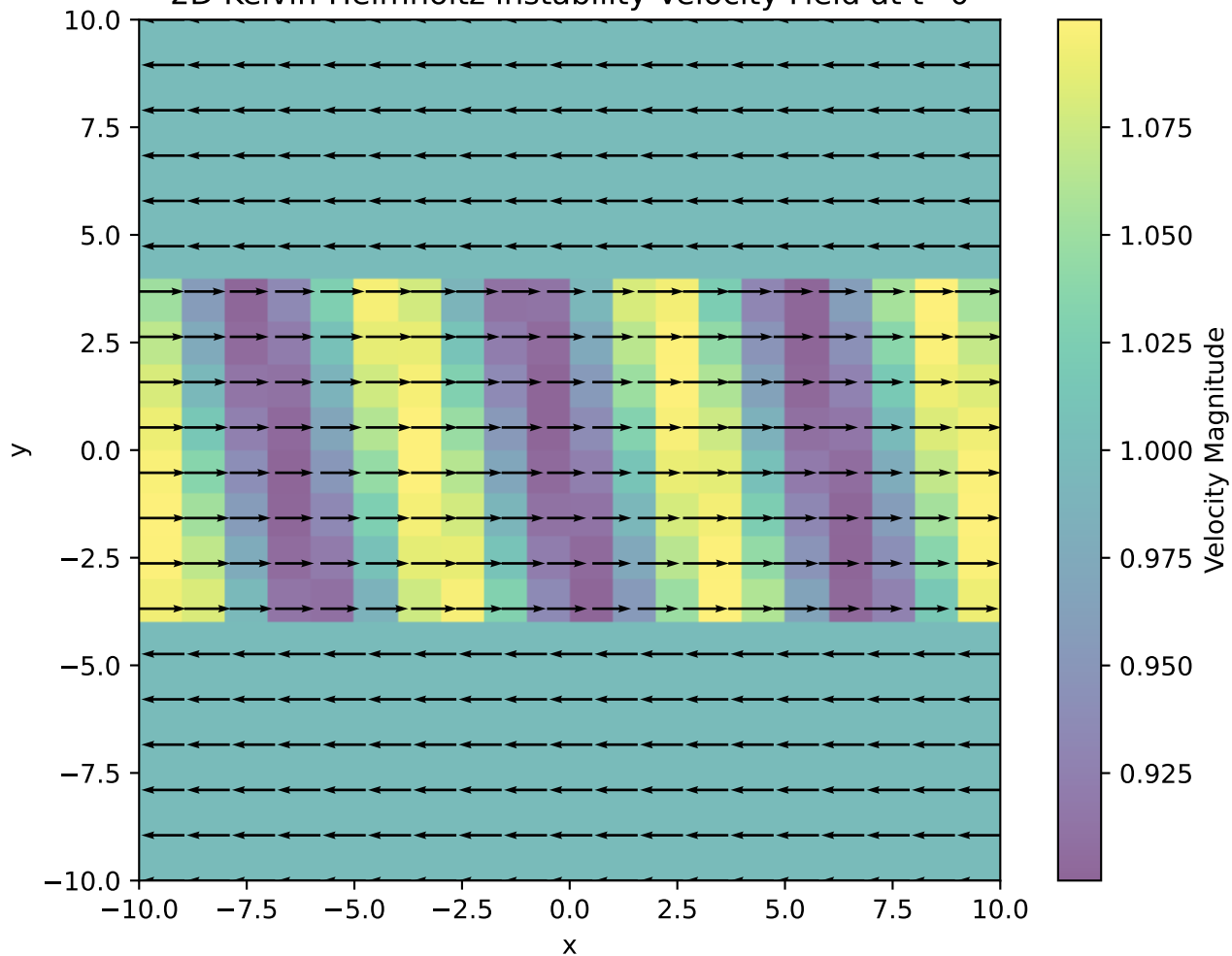
2D Kelvin-Helmholtz instability Velocity Field at t=0
