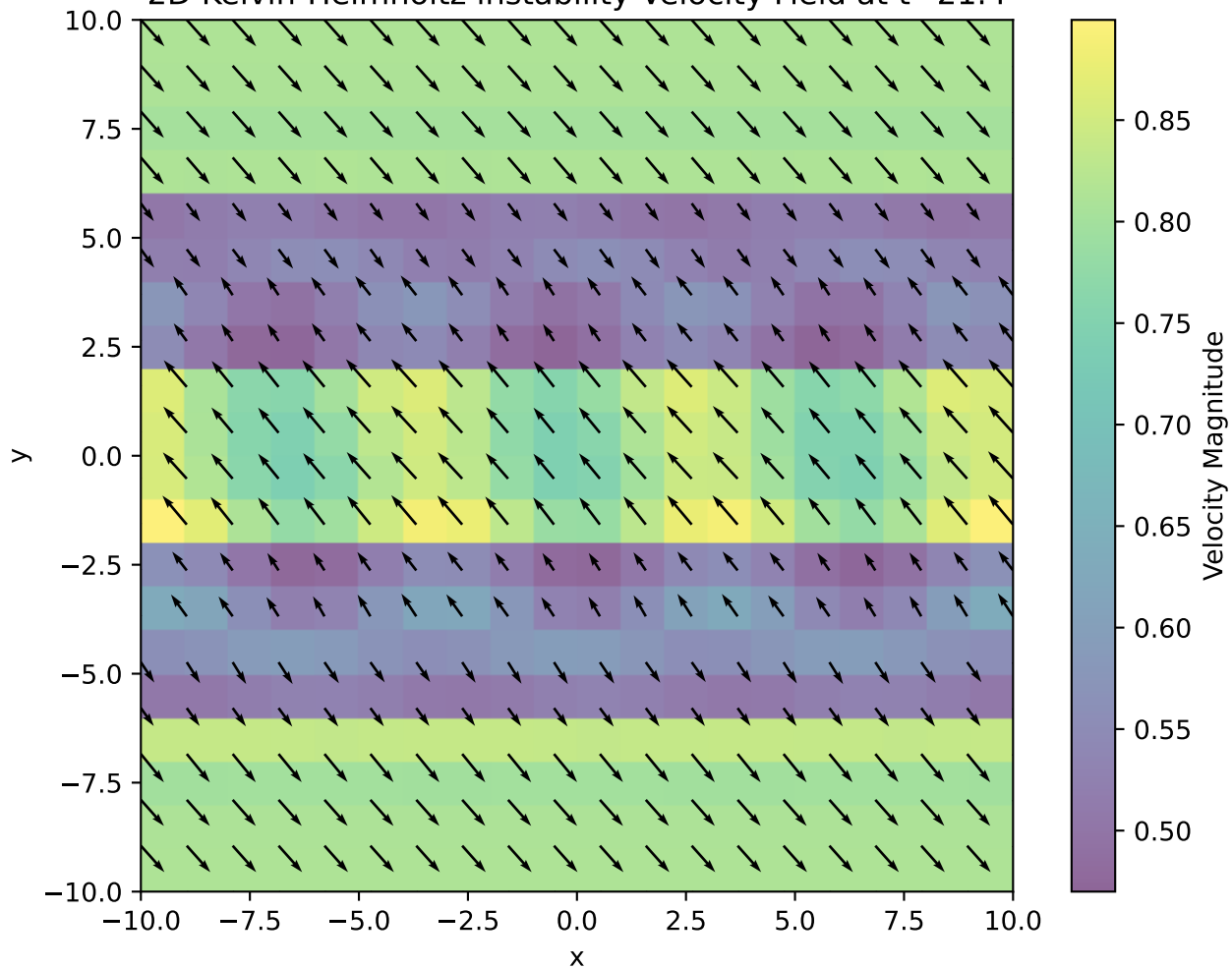
2D Kelvin-Helmholtz instability Velocity Field at t=21.4
