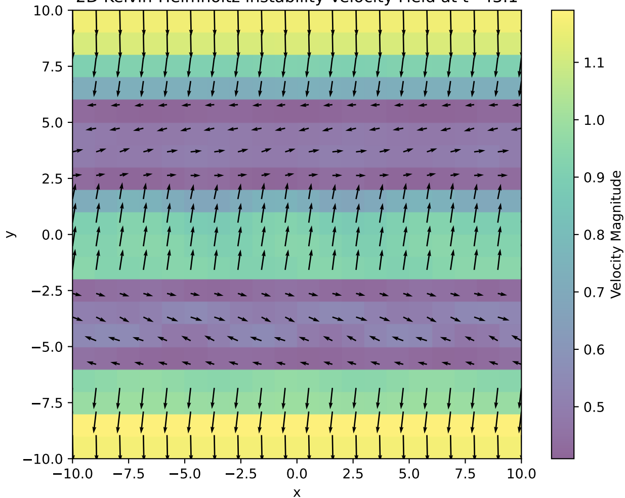
2D Kelvin-Helmholtz instability Velocity Field at t=43.1
