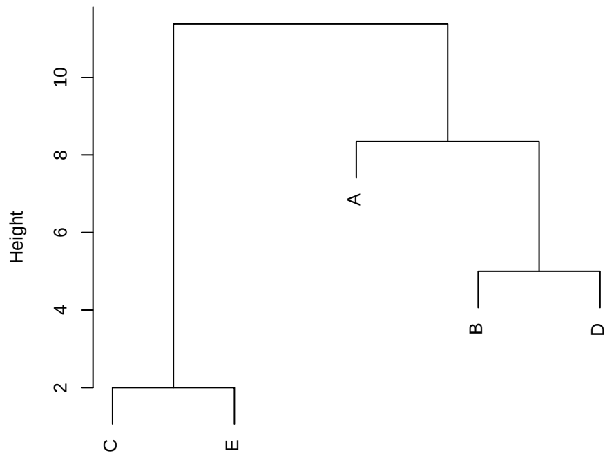
Cluster Dendrogram
