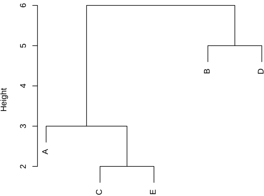
Cluster Dendrogram
