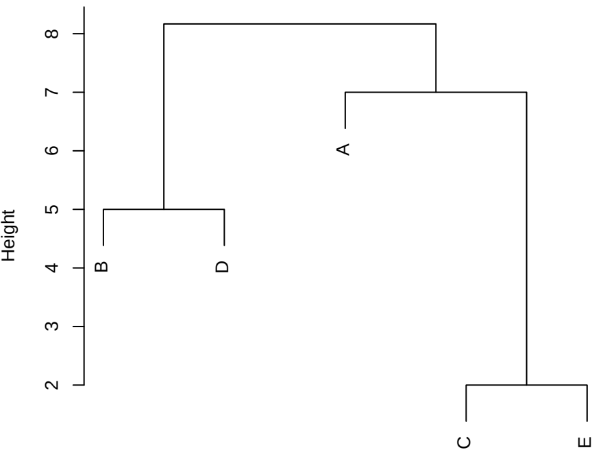
Cluster Dendrogram
