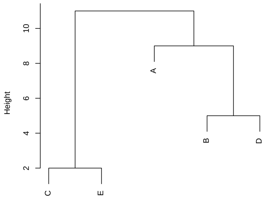
Cluster Dendrogram
