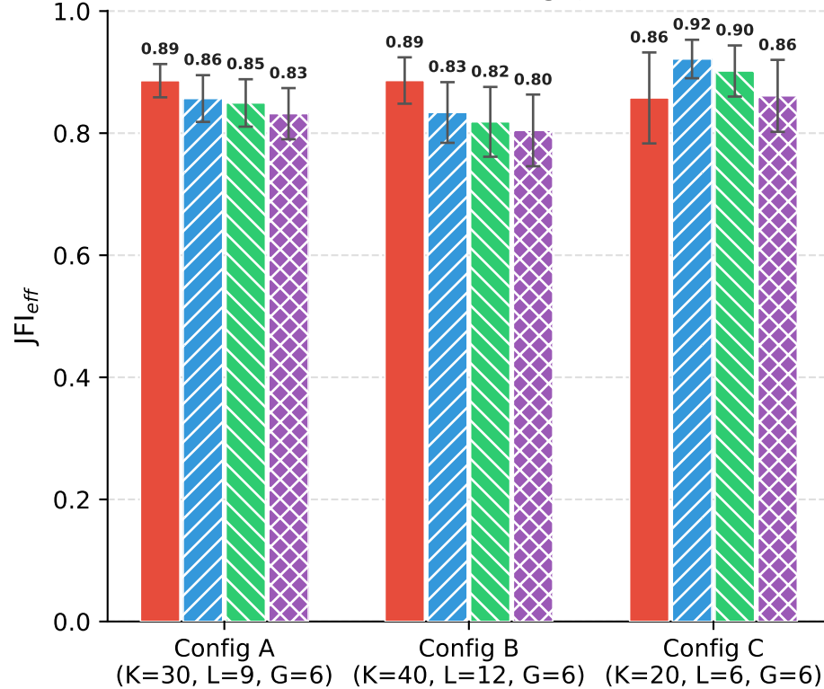
(b) Load Balancing ( JFI_{eff} )
