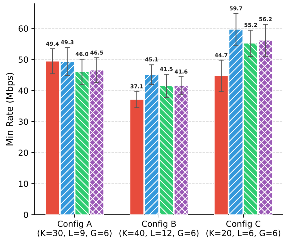
(a) Minimum User Rate
