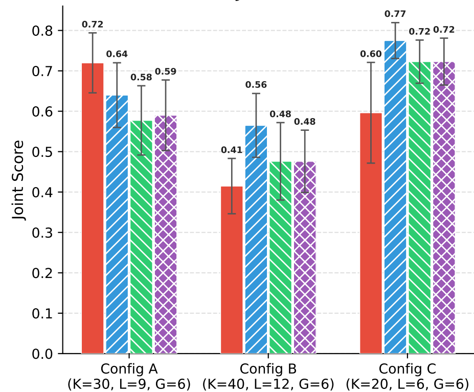
(c) Joint Score
