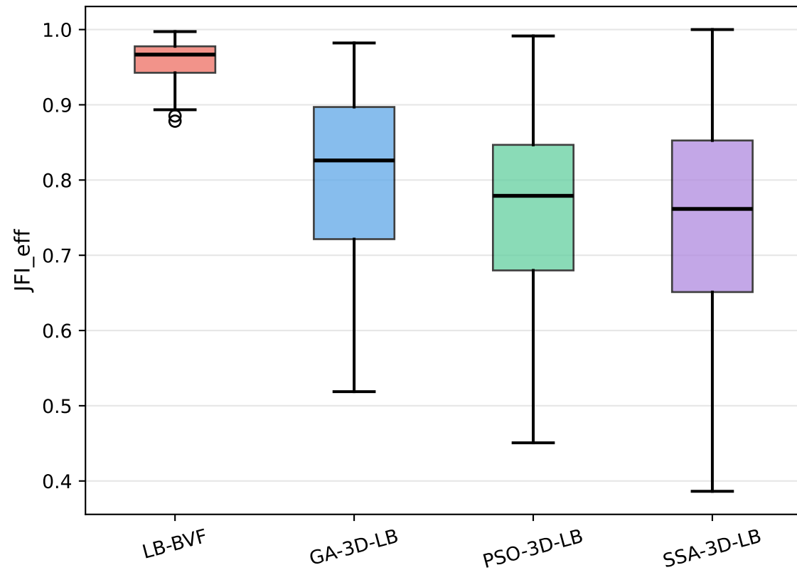
(a) JFI Distribution
