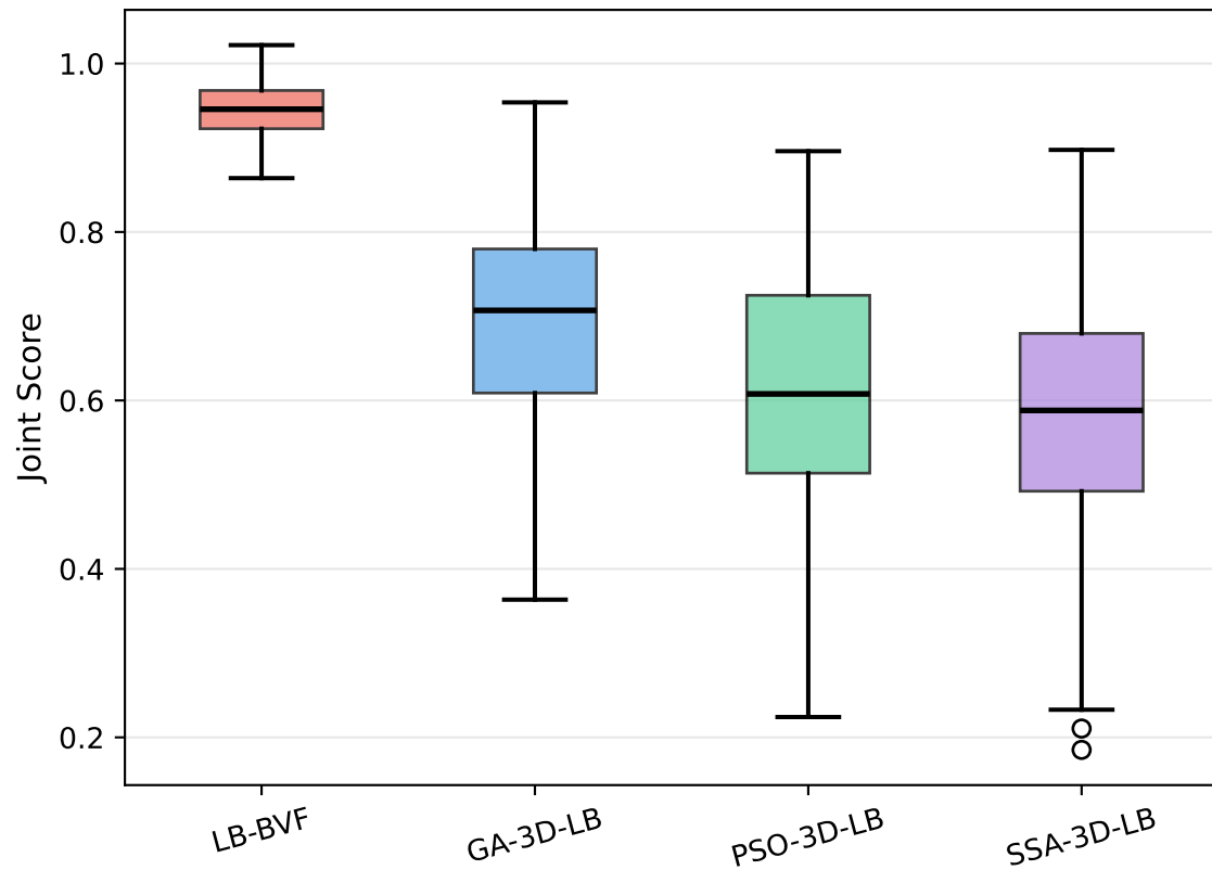
(b) Joint Score Distribution
