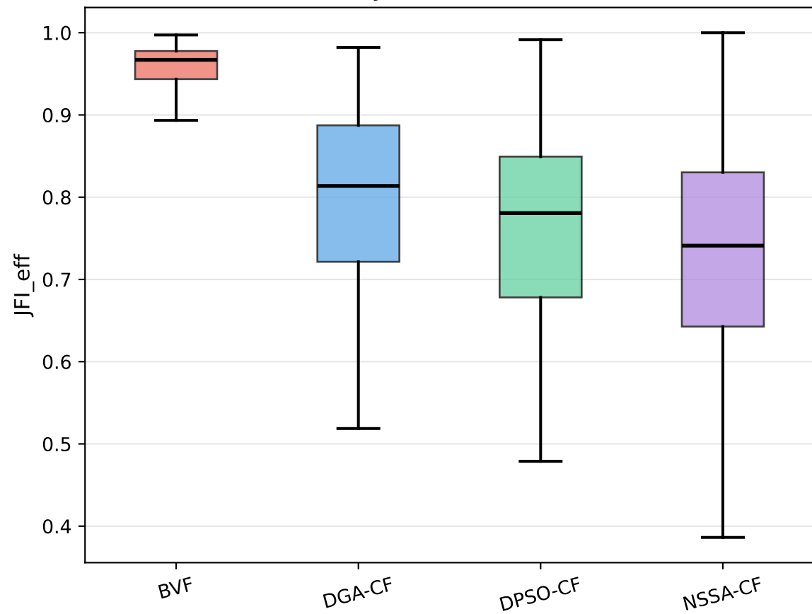
(a) JFI Distribution
