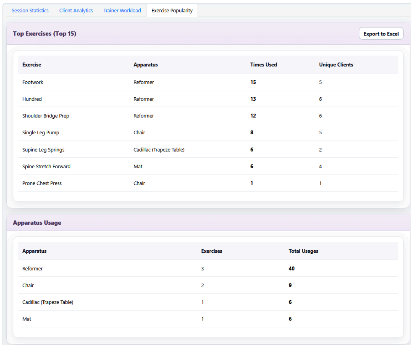
Figure 10. Exercise Popularity tab listing top exercises and apparatus usage.
