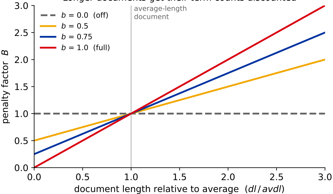
Longer documents get their term counts discounted
