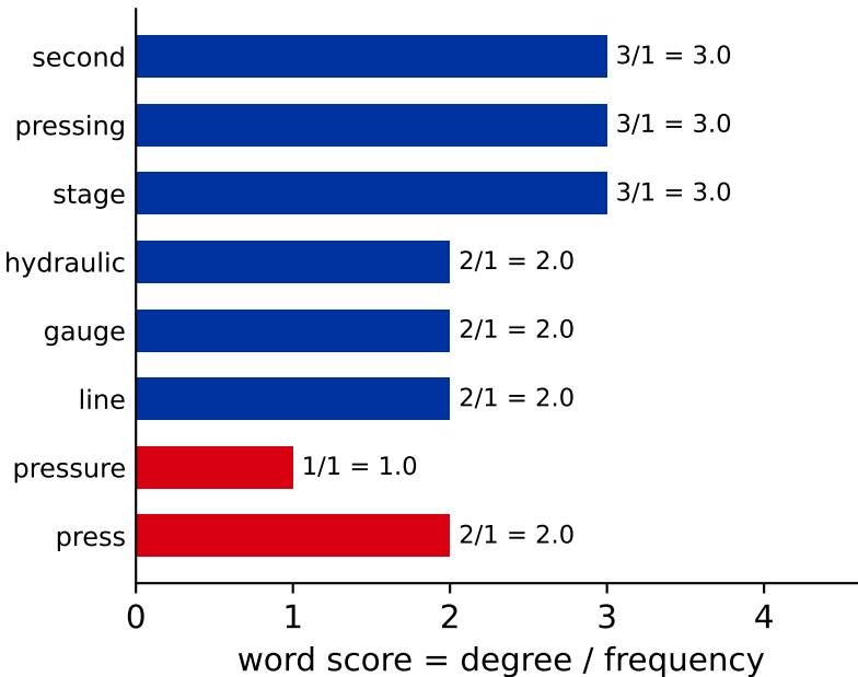
step 1: score each word
