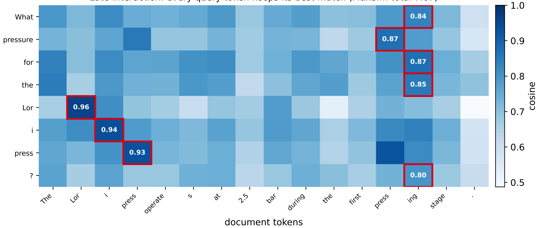
Late interaction: every query token keeps its best match (MaxSim total 7.07)
