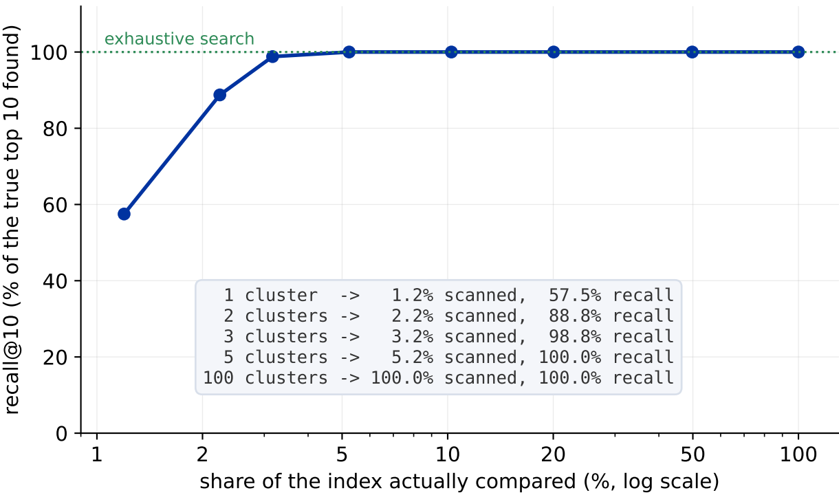
Approximate search: 20,000 vectors in 100 clusters
