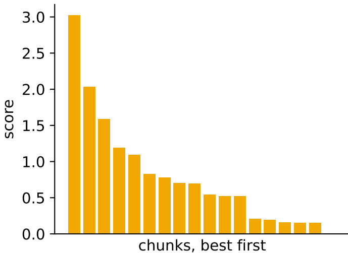
BM25, raw (zeros mean 'no signal')
