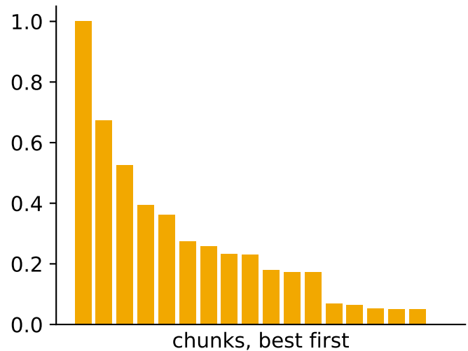
BM25 after min-max (the zeros are now 0.00 too - same number, lost meaning)
