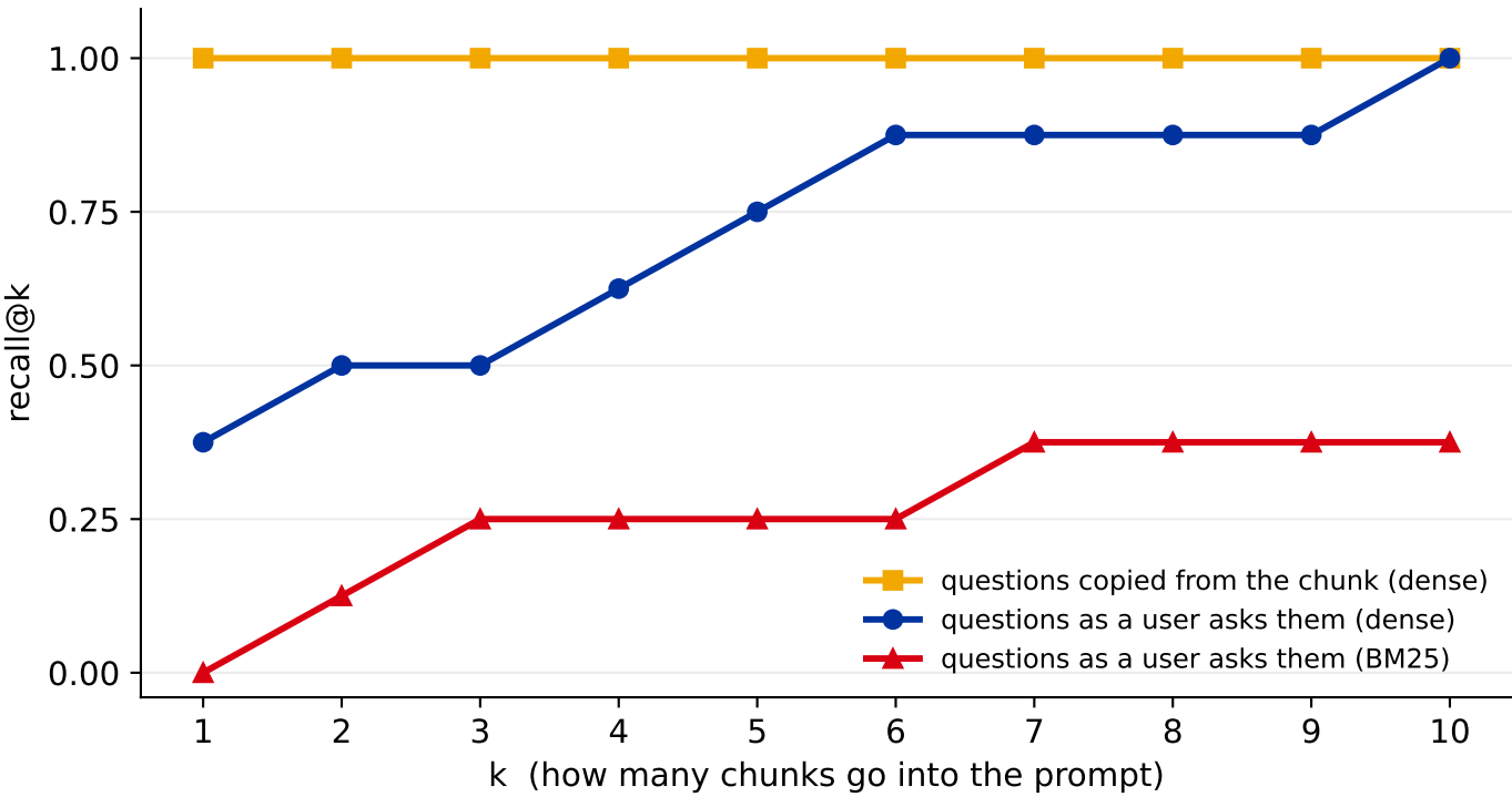
8 questions, 20 chunks, one correct chunk each
