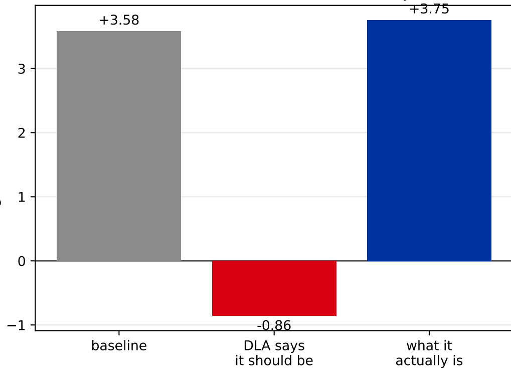
Delete the three heads that do the job
