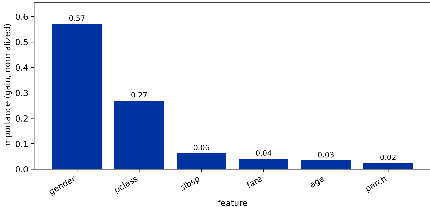
Gain-based feature importance (XGBoost on Titanic)
