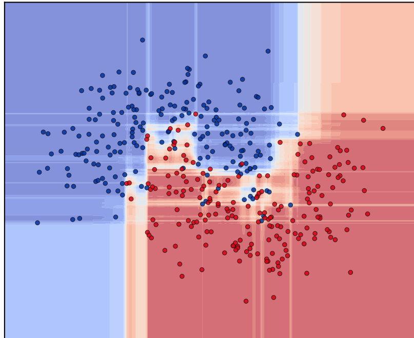
random forest (300): smoother
