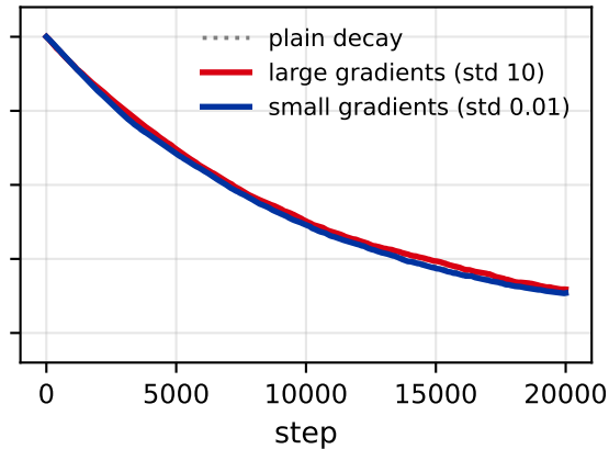
AdamW(weight_decay=0.1)
