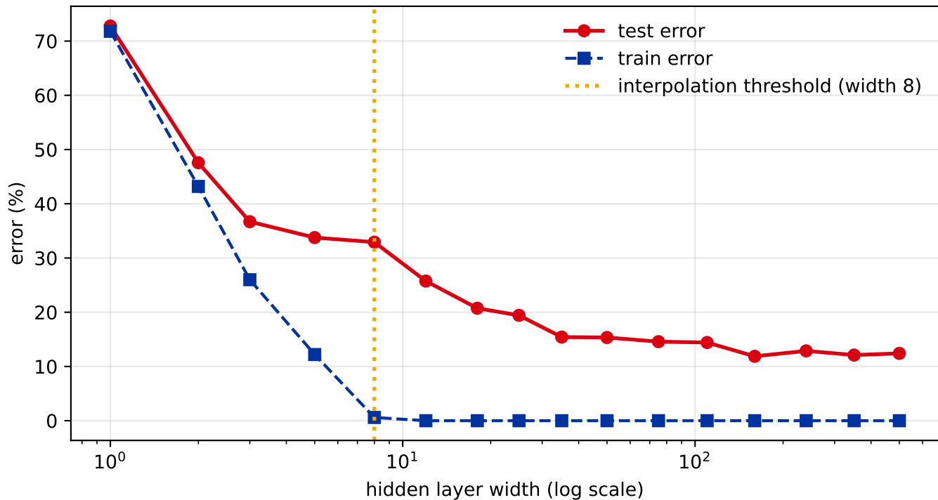
Double descent: 500 digits, 15% label noise
