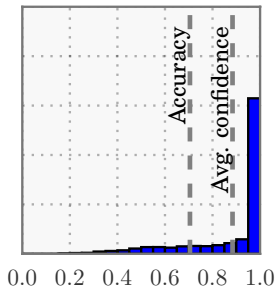
ResNet (2016) CIFAR-100
