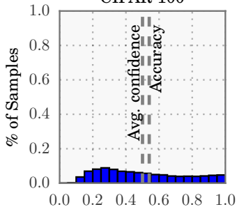
LeNet (1998) CIFAR-100
