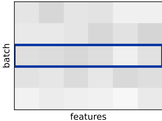
LayerNorm
