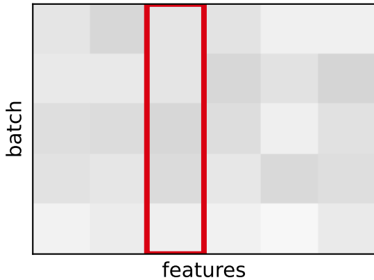
BatchNorm
