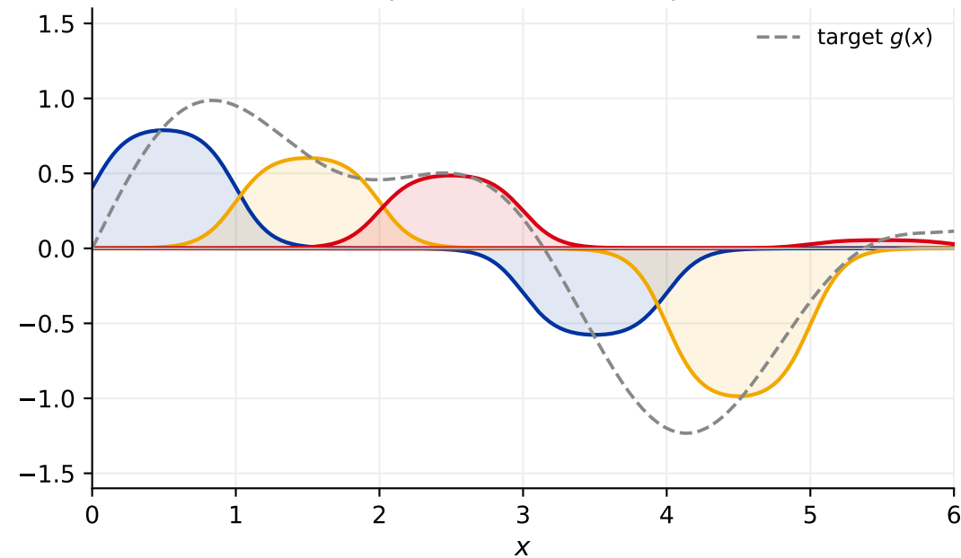
Each neuron pair adds one bump (6 shown)
