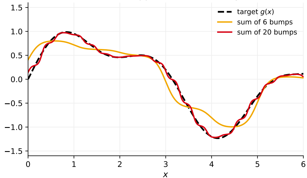
Their sum approximates the target
