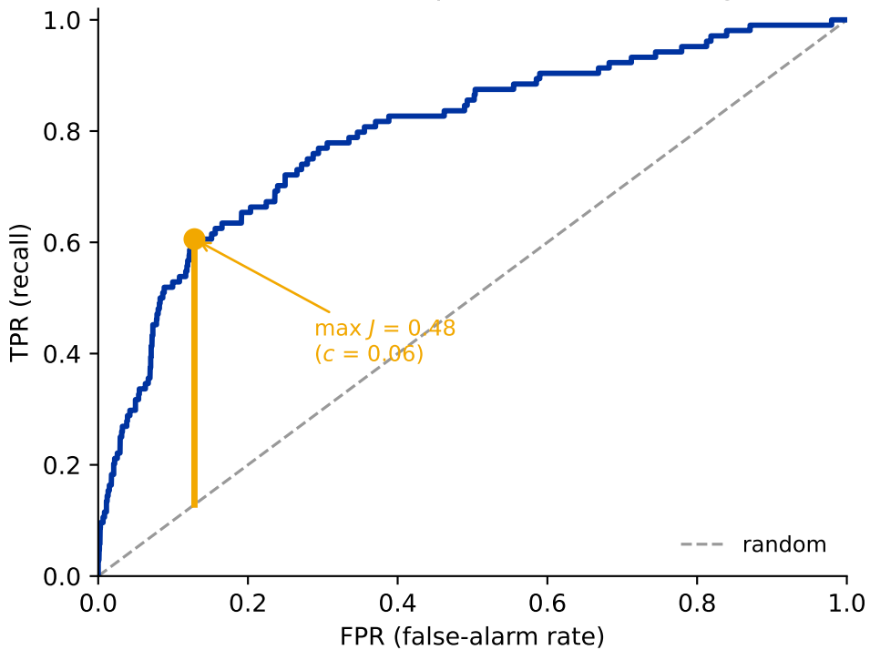
Youden's J: farthest point above the diagonal
