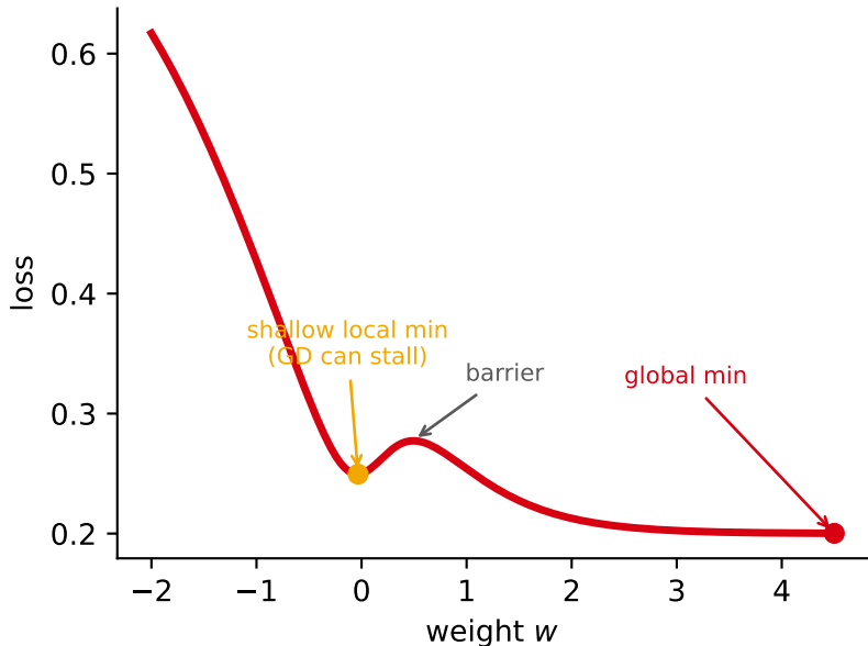
squared loss on sigmoid: non-convex
