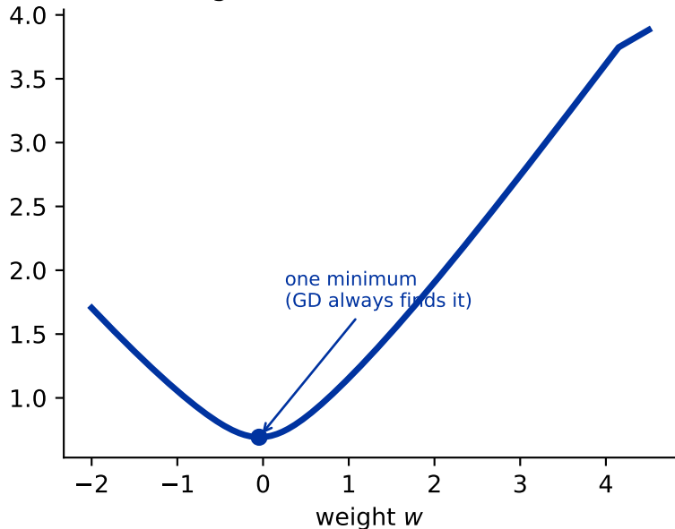
log-loss: one convex bowl
