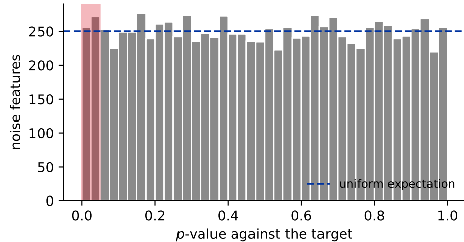
10,000 columns of pure random numbers
