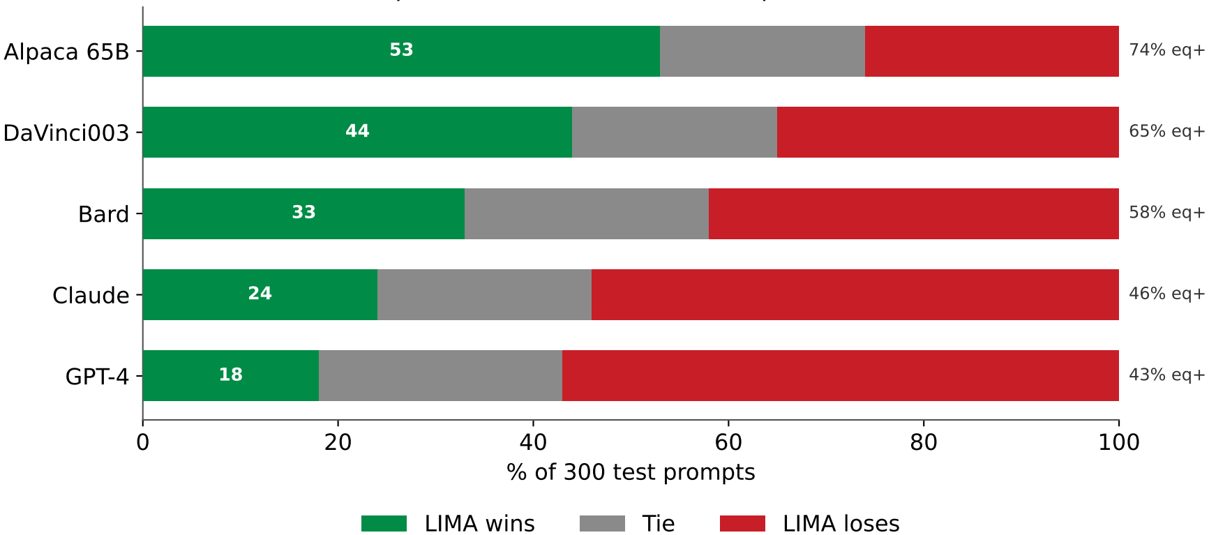
Human preference: LIMA (1,000 examples) vs the field
