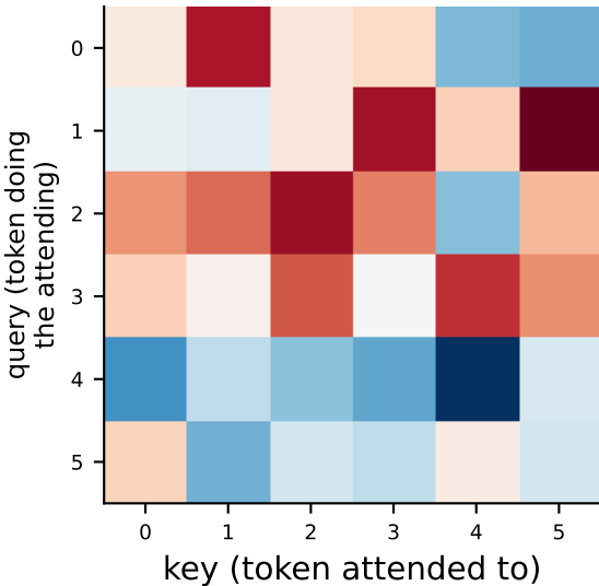
raw scores QK^T/\sqrt{d_k}
