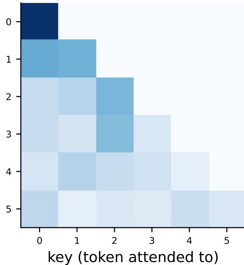
after softmax: rows sum to 1
