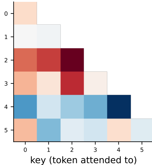
after adding -\infty above the diagonal
