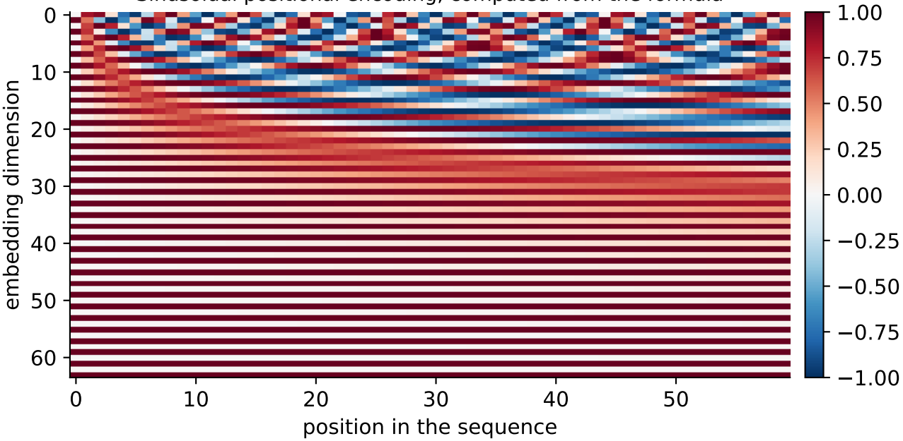
Sinusoidal positional encoding, computed from the formula
