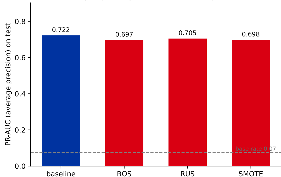
Resampling barely moves the ranking (PR-AUC)
