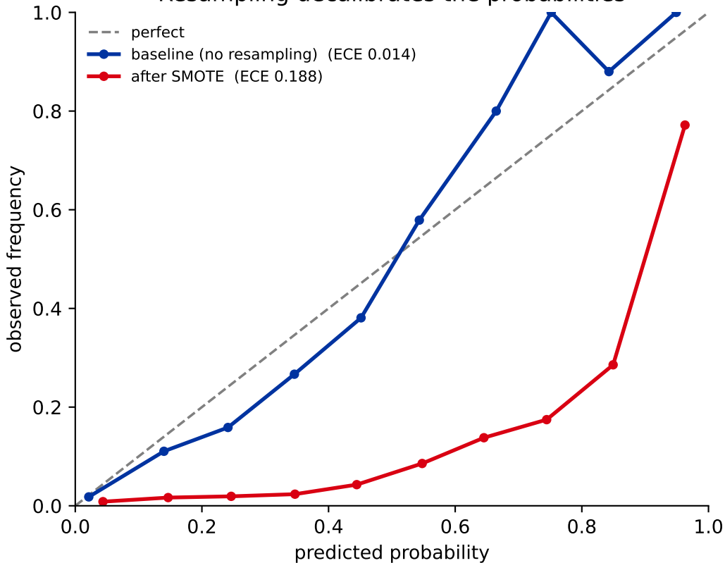
Resampling decalibrates the probabilities
