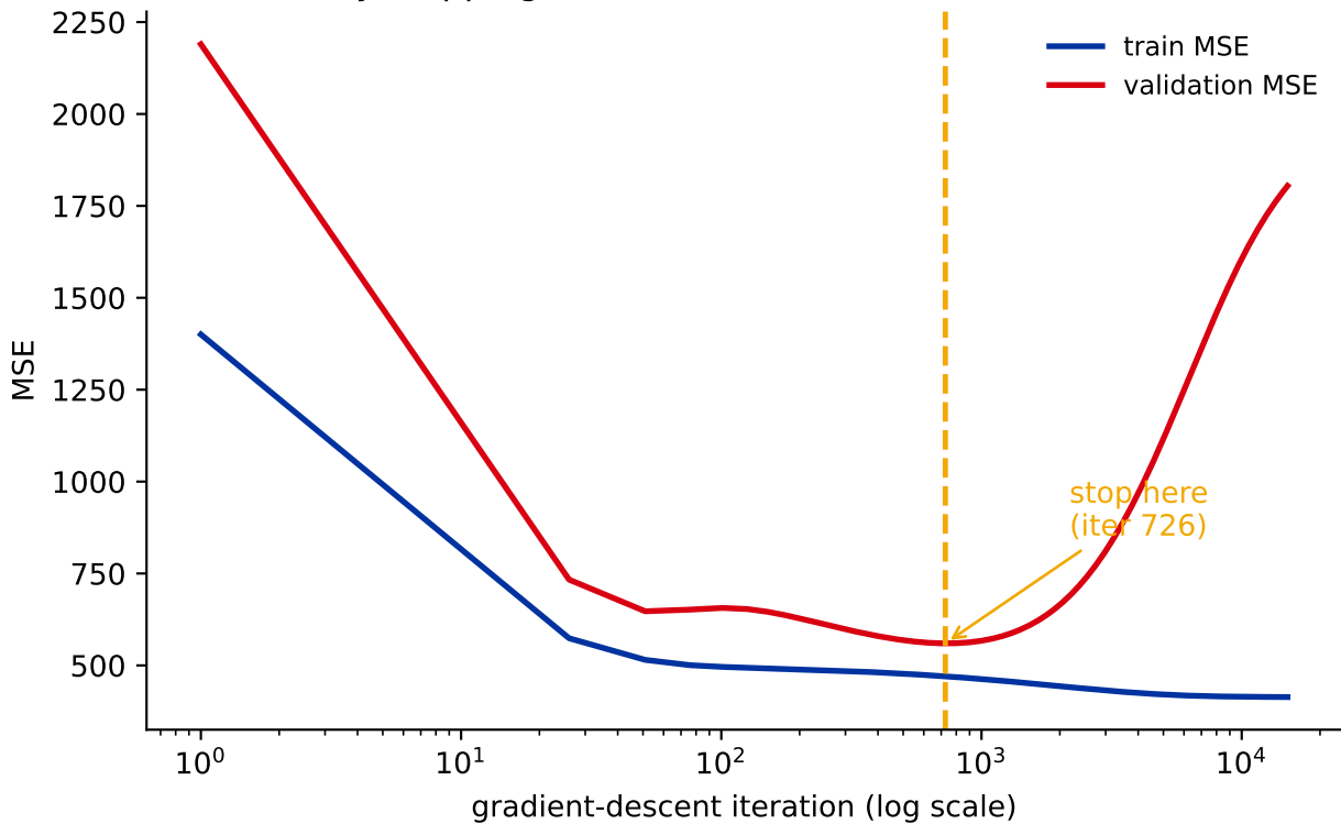
Early stopping: the validation curve has a minimum
