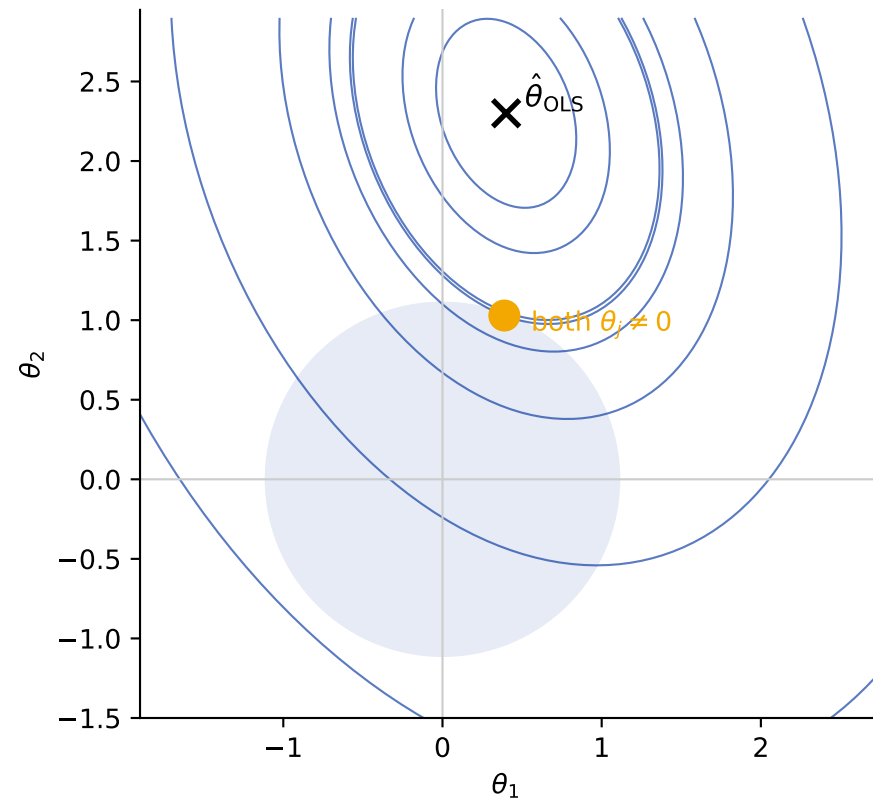
Ridge ( L_2 ): round ball \Rightarrow no zeros
