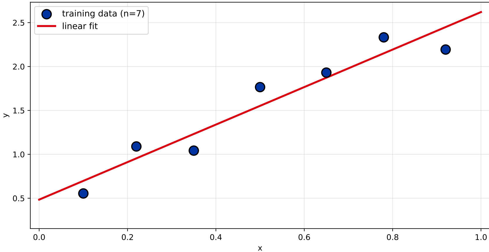
Linear fit on 7 points -- train MSE = 0.032
