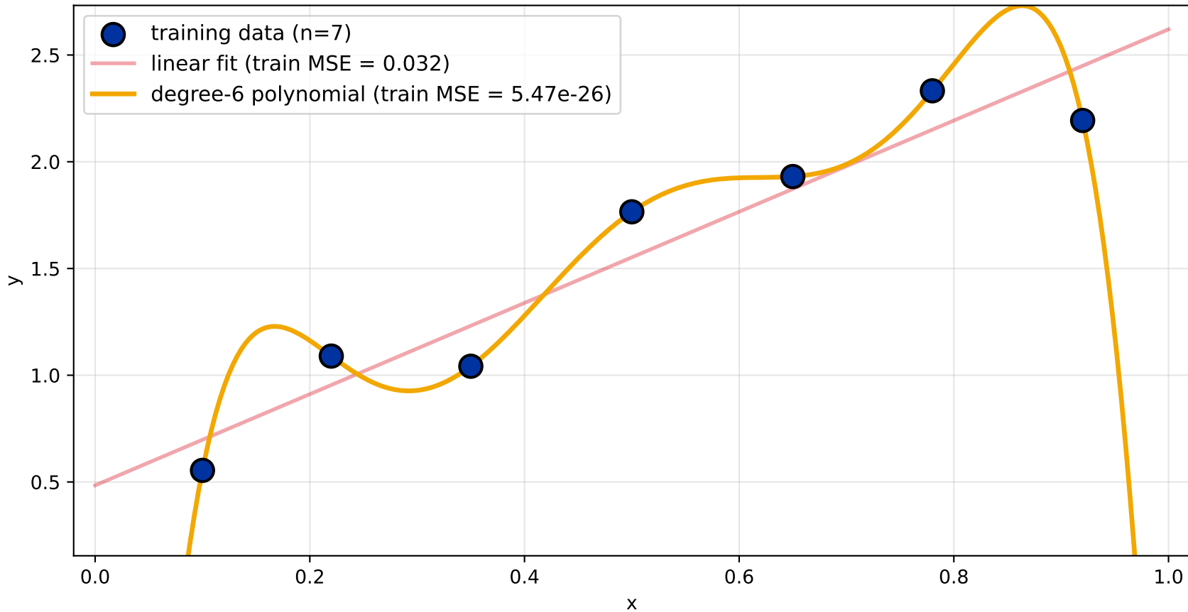
Degree-6 polynomial: zero training error
