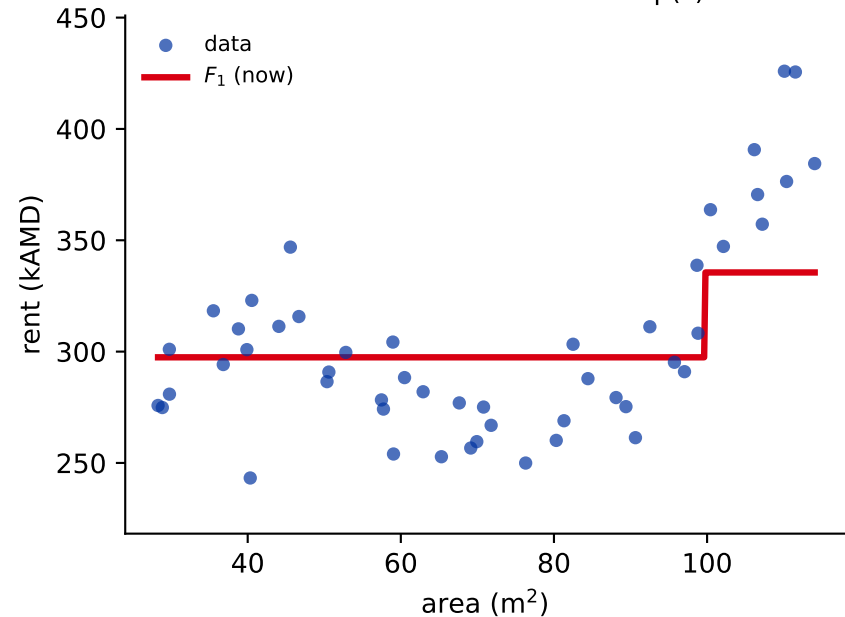
round 1: ensemble of 1 stump(s)
