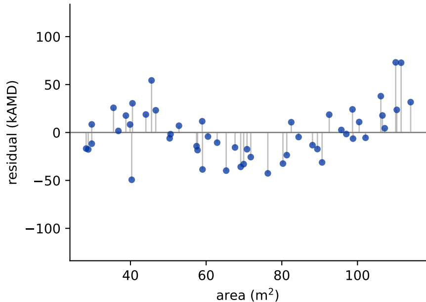
what's left: residuals r_2 = y - F_2
