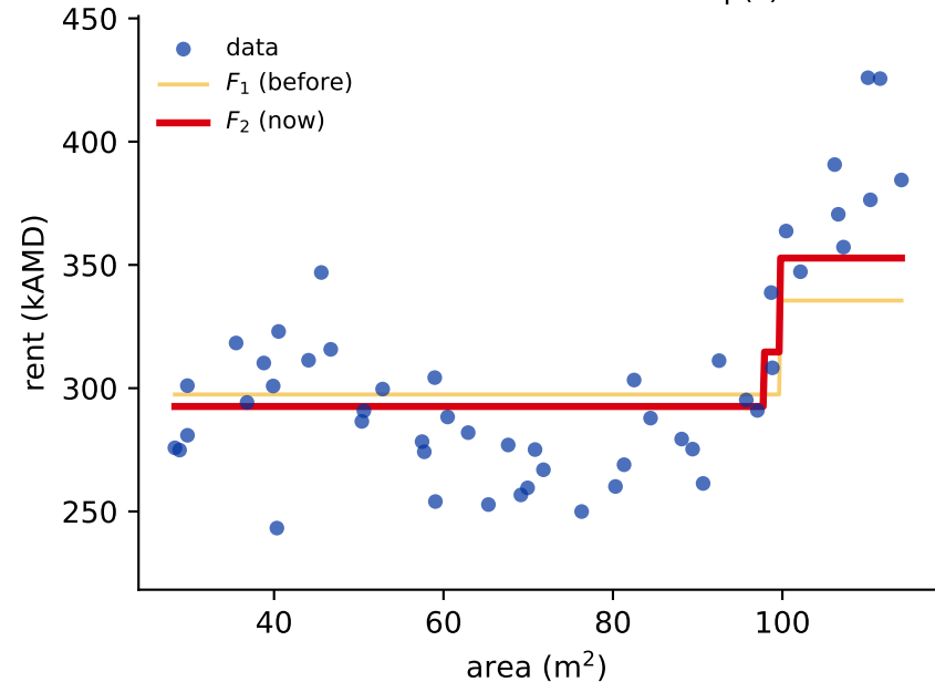
round 2: ensemble of 2 stump(s)
