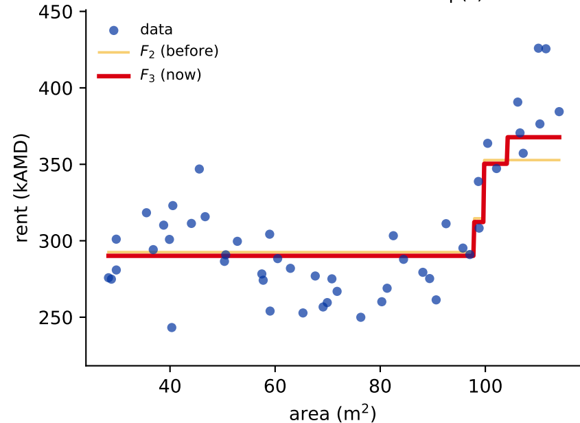
round 3: ensemble of 3 stump(s)
