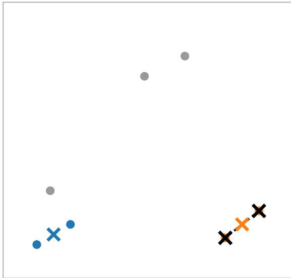
merge 2: nearest midpoints, d = 0.64
