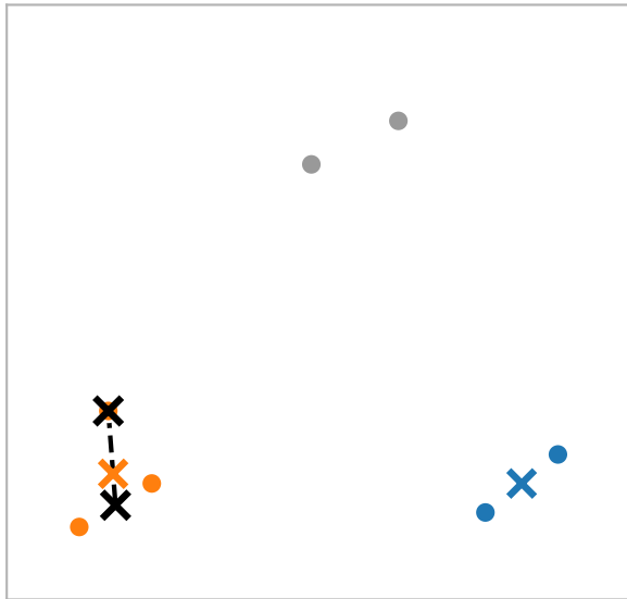
merge 3: nearest midpoints, d = 0.65
