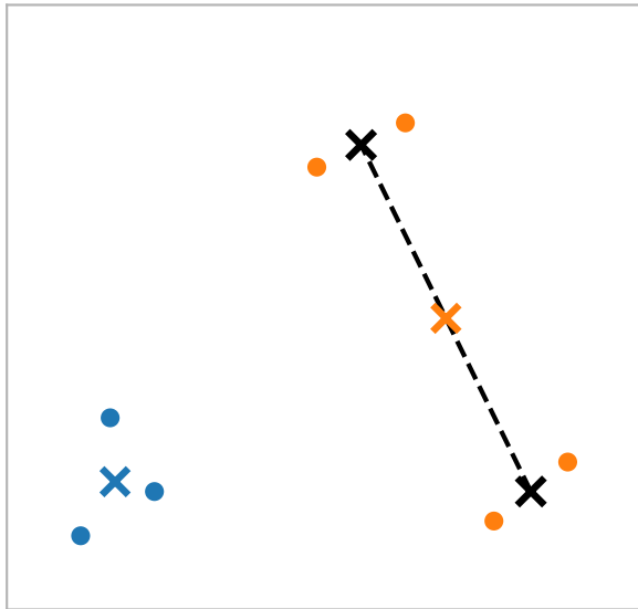
merge 5: nearest midpoints, d = 2.62
