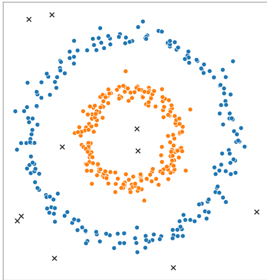
DBSCAN: finds the rings (x = noise)
