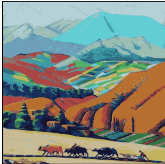
k-means, 16 colors
