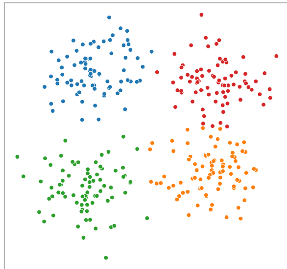
the clustering
